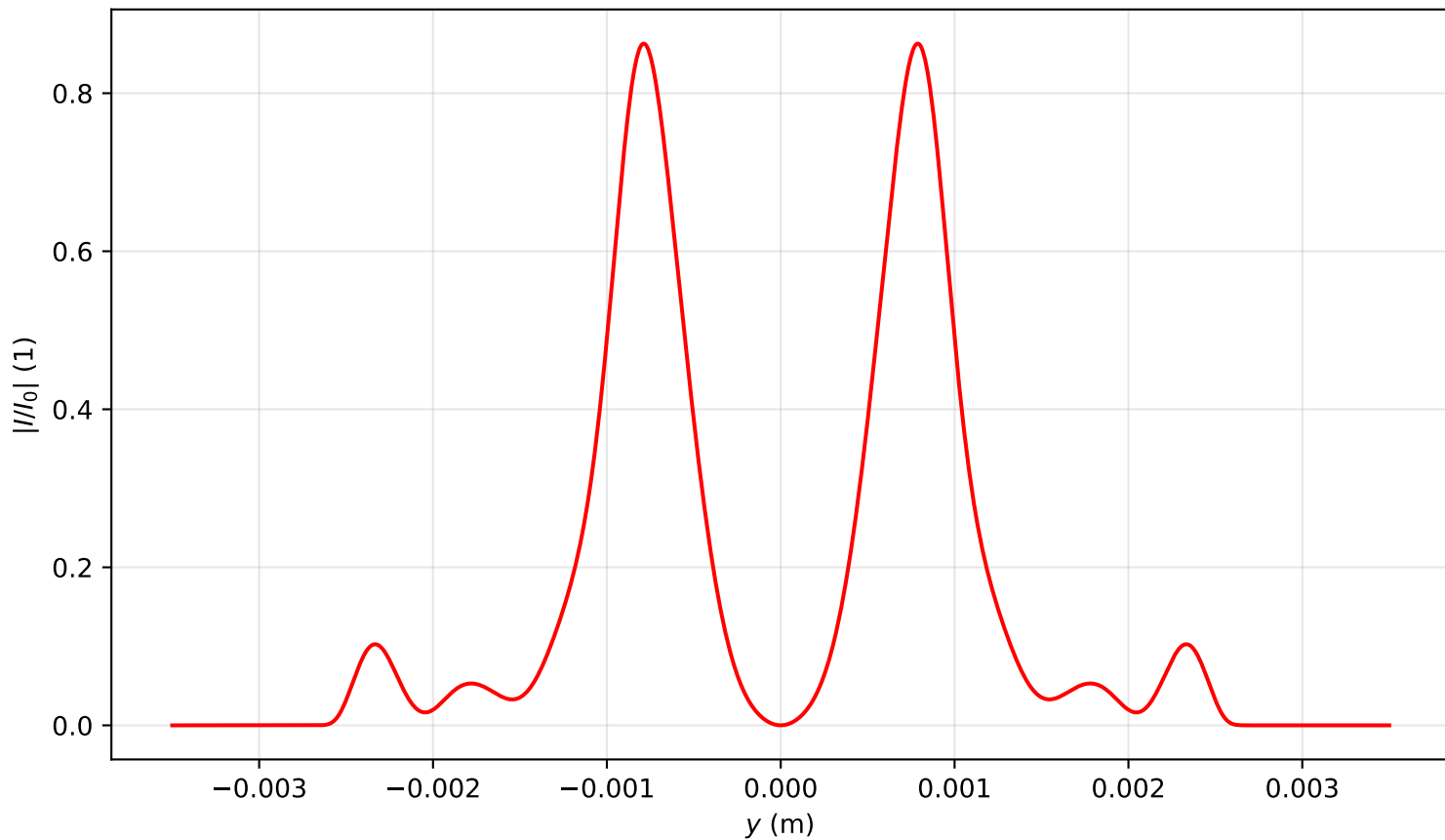
Intensity profile I(x=0, y, z=3.742)/I_0 , P_{in}=5.0P_{cr} , artificial time
